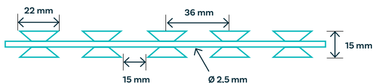
BTO 22 dimensions
