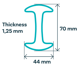
Post section
