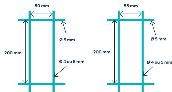
Sizes of compatible fence panels
