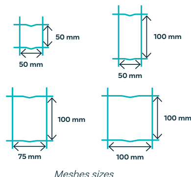
Meshes sizes
