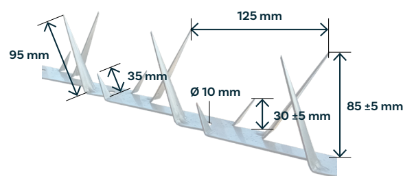
Medium wall spikes dimensions
