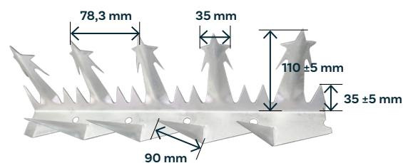
Heavy wall spikes dimensions
