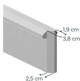
Compatible with Ritmo post
