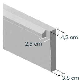
Compatible with Bekafix post
