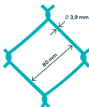
Mesh diagram
