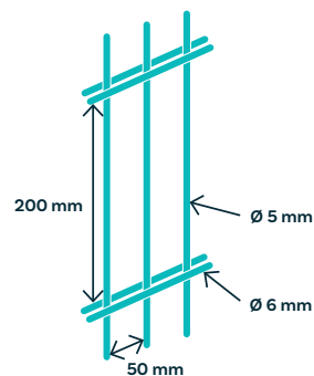
Panneau Ø 6/5/6
